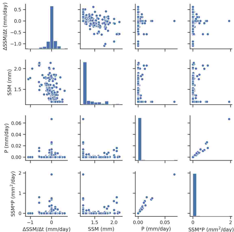
Figure C1. Pairwise scatter plot of the dependent variable and regressors constructed in Regression Form II from SMAP/IMERG data at an example pixel (23.98°N, 23.71°E) in Sahara with collinearity.
